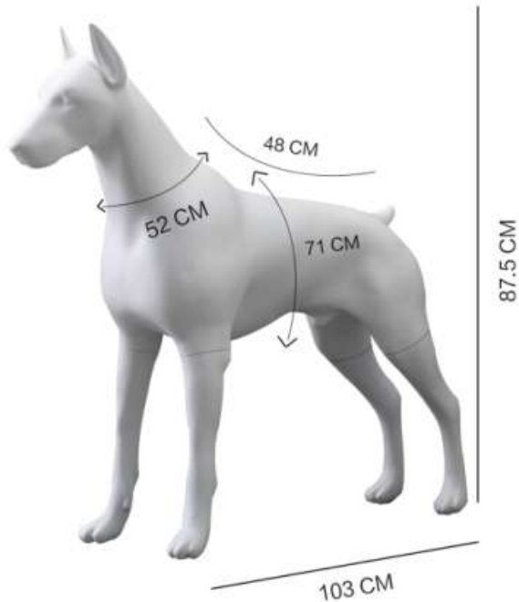
Dober-A Height: 87.5 cm Length: 103 cm Neck: 52cm Chest: 71cm Back: 48cm Material: fiberglass Color: Matte white Split: Four legs detachable CTN.: 97*32*60cm N.W: 5.6KG G.W: 7.7KG
